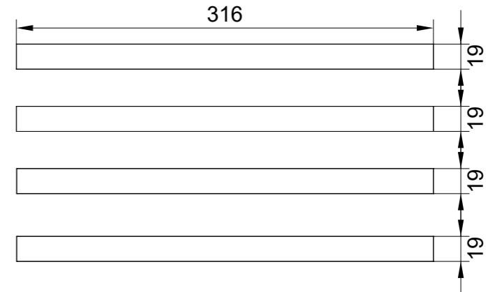
Baffle & Rear Panel Mounting Cleats (19mm solid pine):
