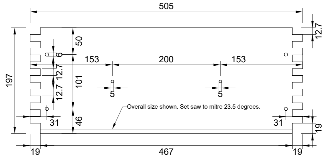
Top (19mm solid pine):
