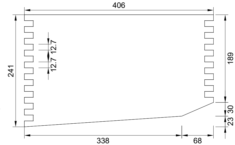
RH End (19mm solid pine):
