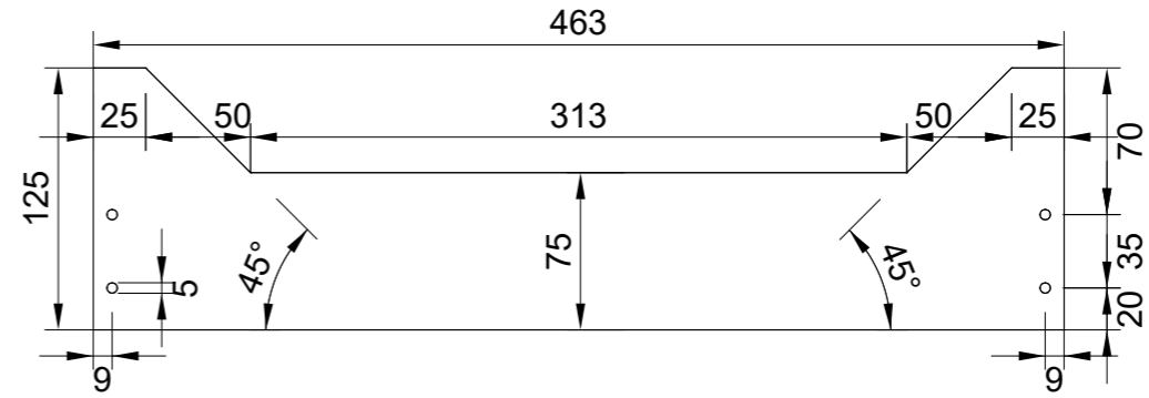
Upper Back Panel (9mm ply):
