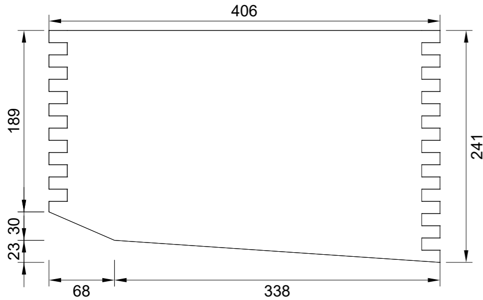
Baffle (9mm ply):
