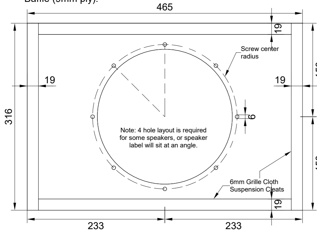
Baffle (9mm ply):
