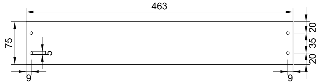
Lower Back Panel (9mm ply):
